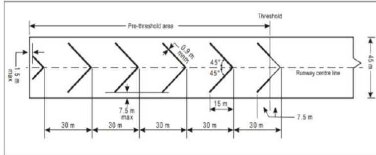
Figure 7-2. Pre-threshold marking
