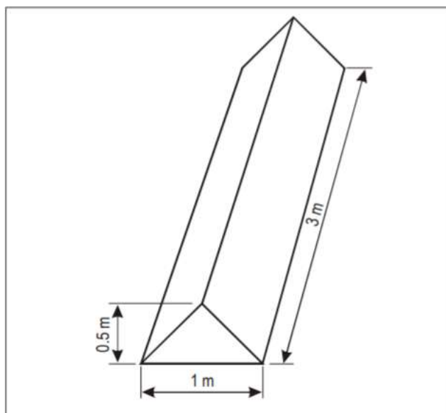
Figure 5-34 Boundary Markers
