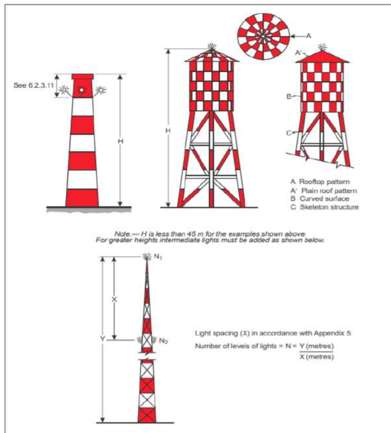
Figure 6-2: Marking and lighting of tall structures
